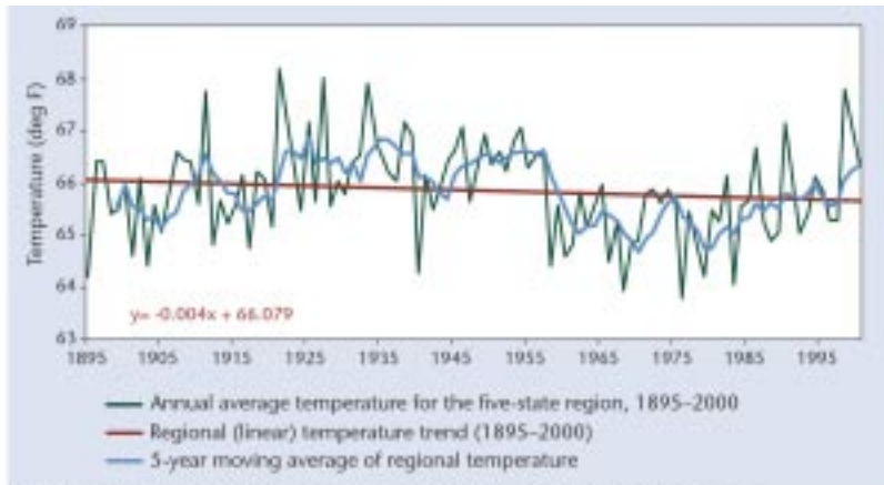
FIGURE 4 Gulf Regional Average Temperature (1895–2000)
